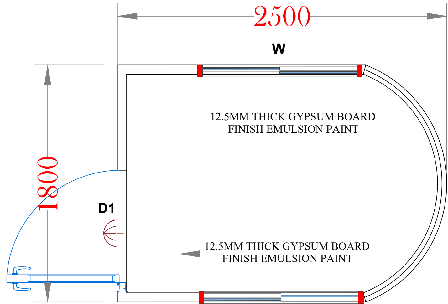
CEILING PLAN
