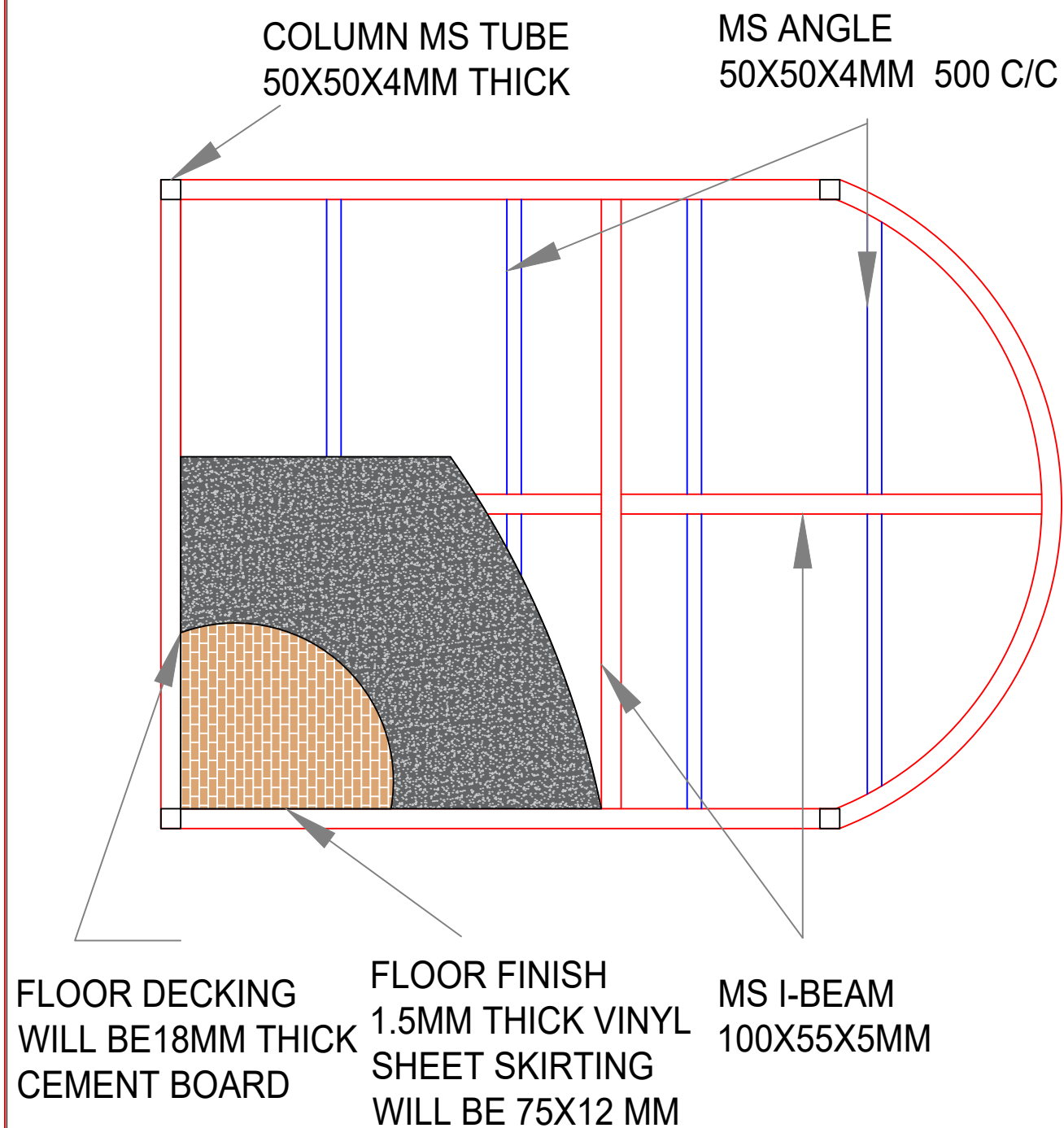
BASE FRAME
