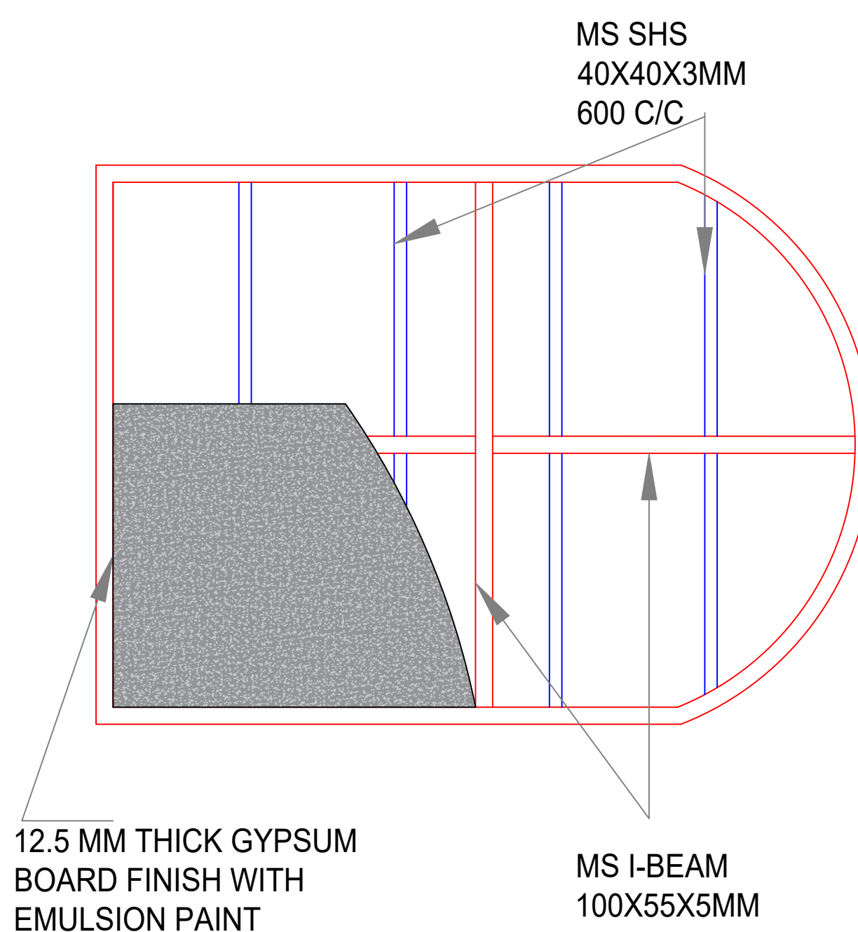
TOP FRAME
