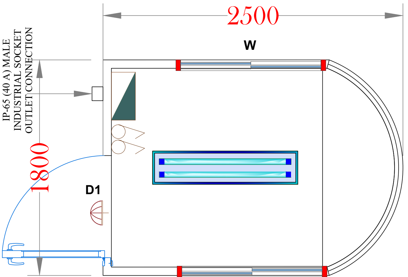
LIGHTING PLAN
