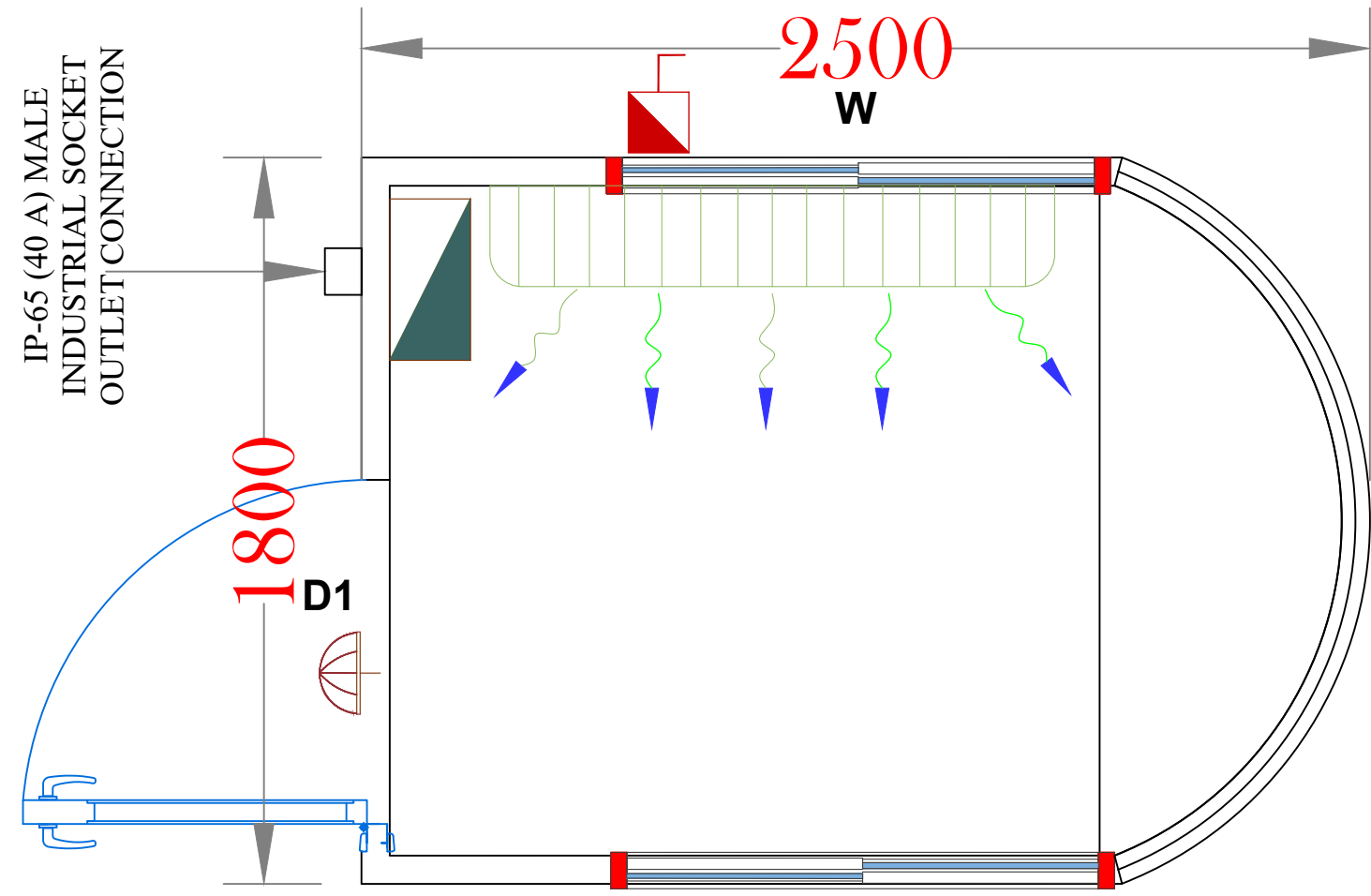
AC LAYOUT
