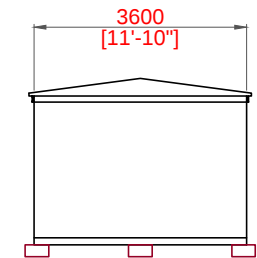
RIGHT SIDE ELEVATION
