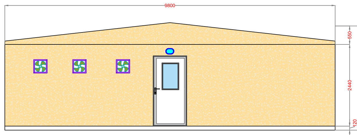
ELEVATION "D"
