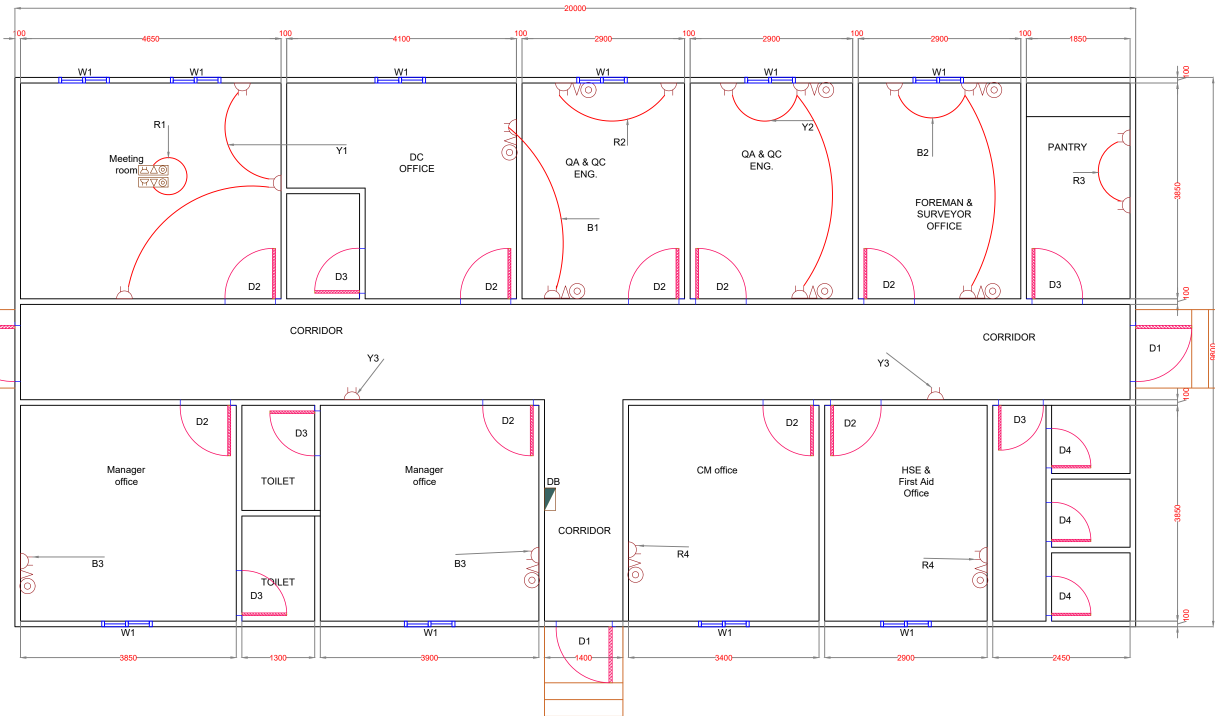
POWER LAYOUT
