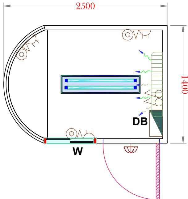
FLOOR PLAN
