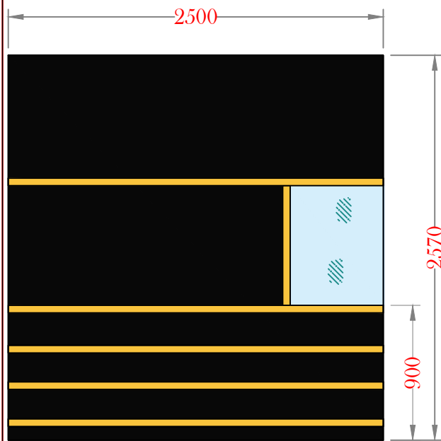
LEFT ELEVATION
