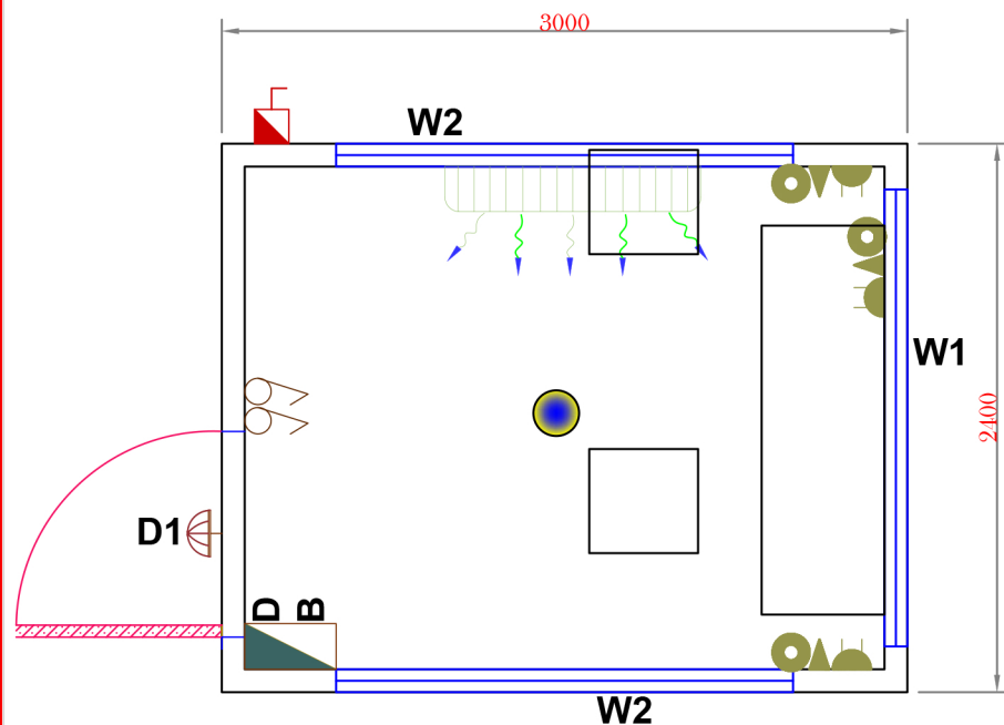
FLOOR LAYOUT
