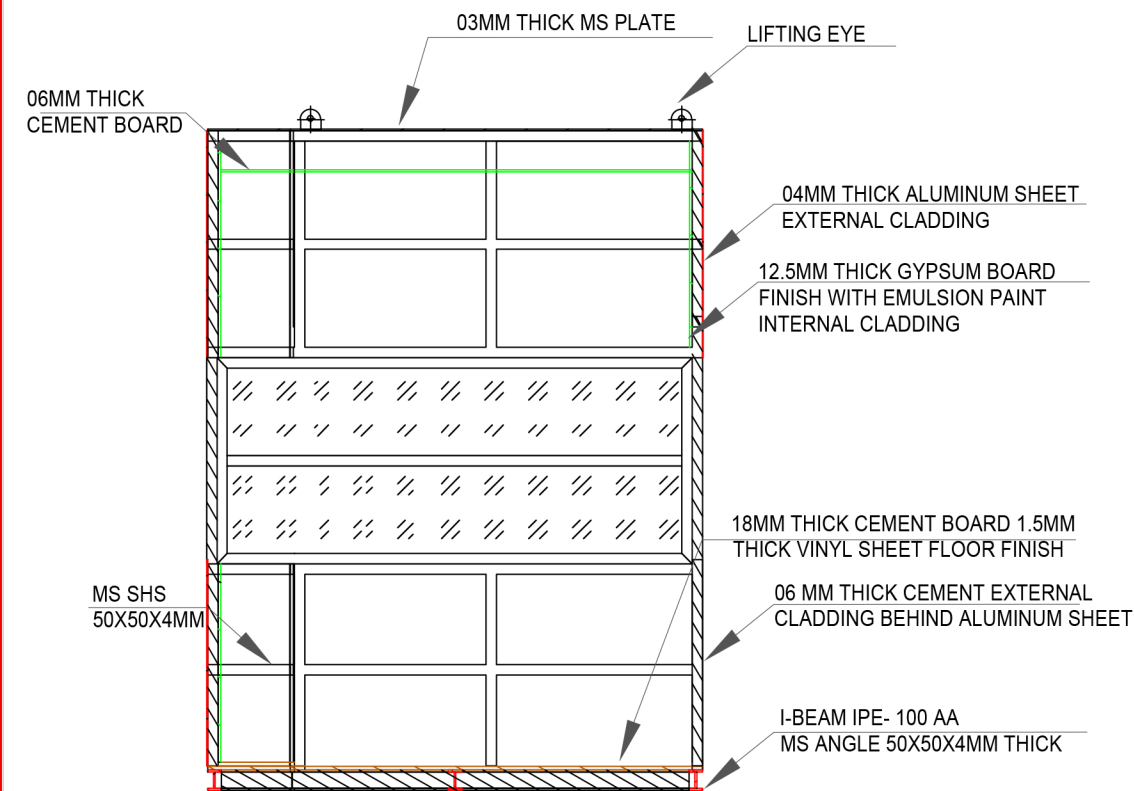
SECTION DETAIL
