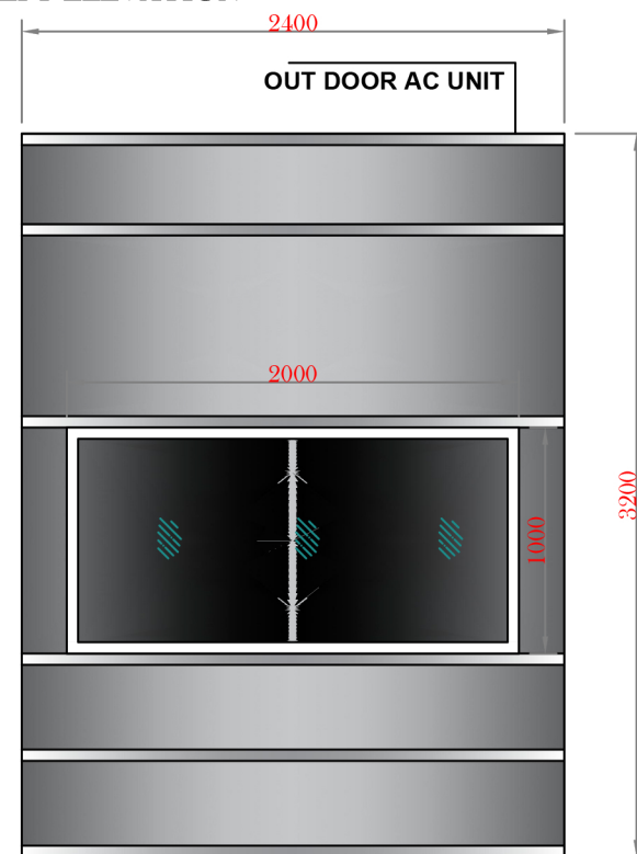
FRONT ELEVATION
