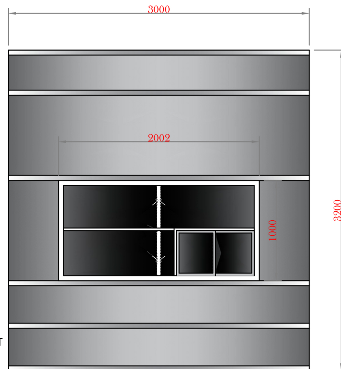
LEFT ELEVATION
