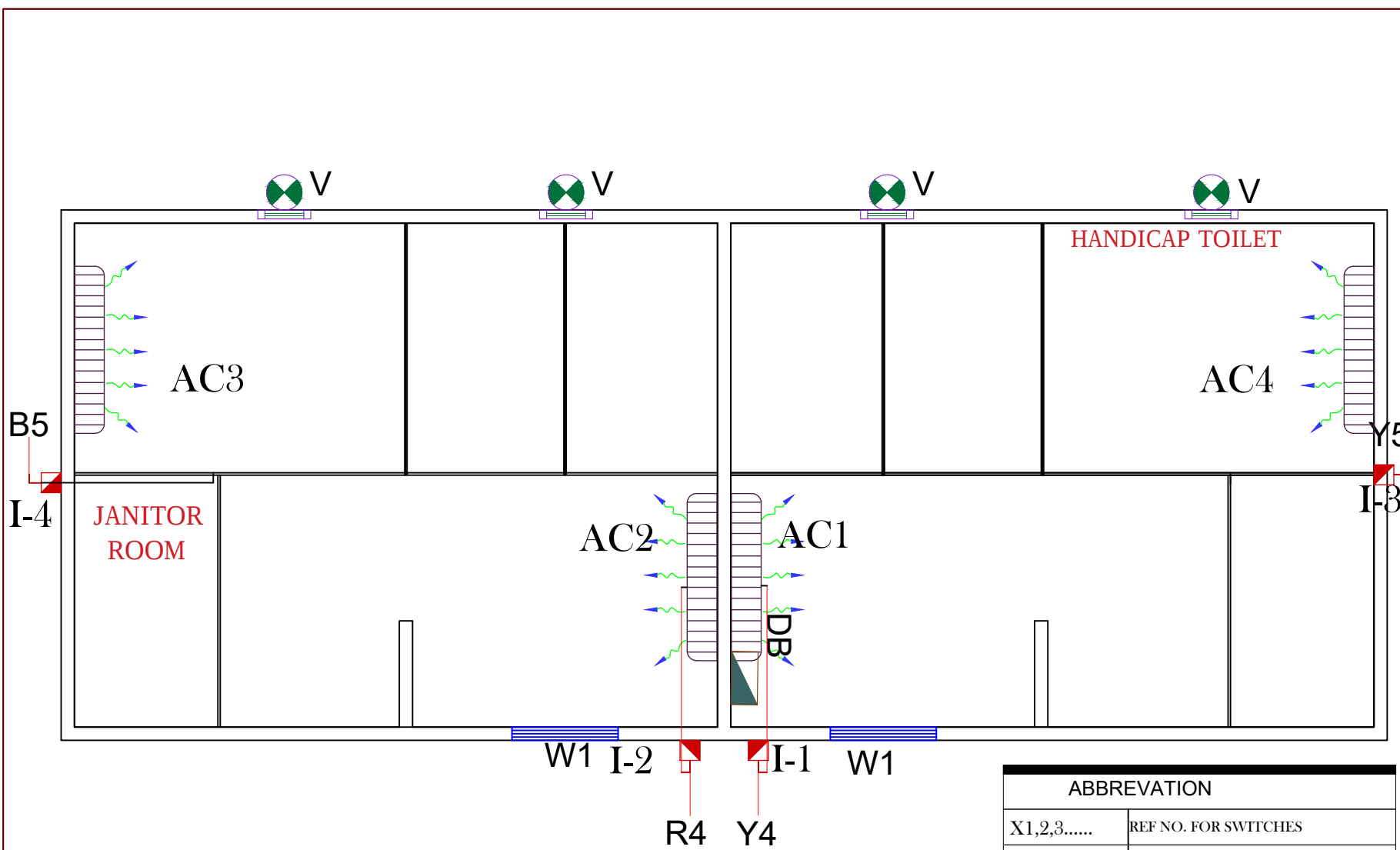
AC LAYOUT
