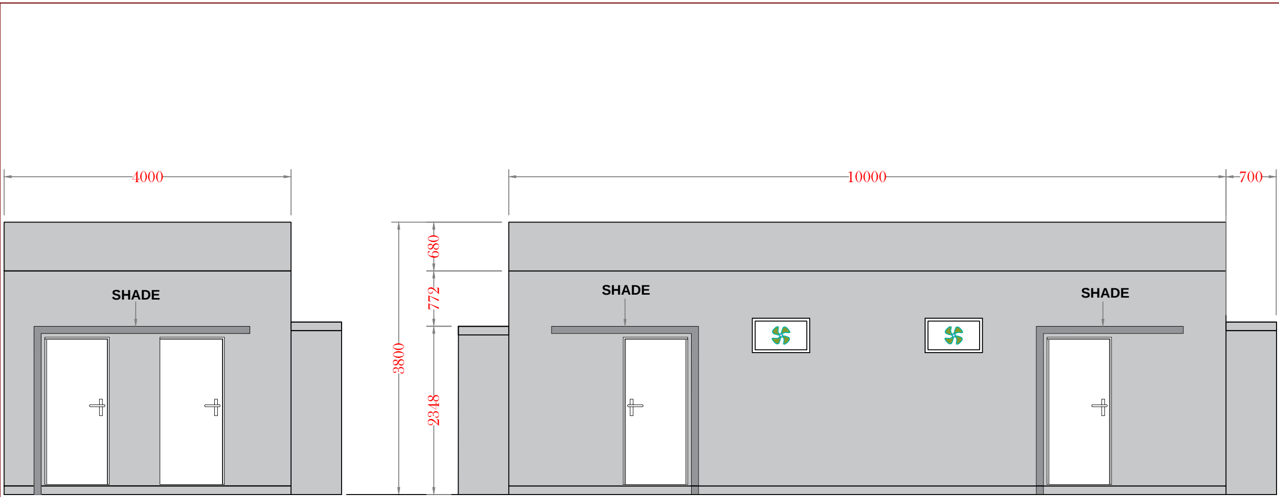
LEFT ELEVATION
