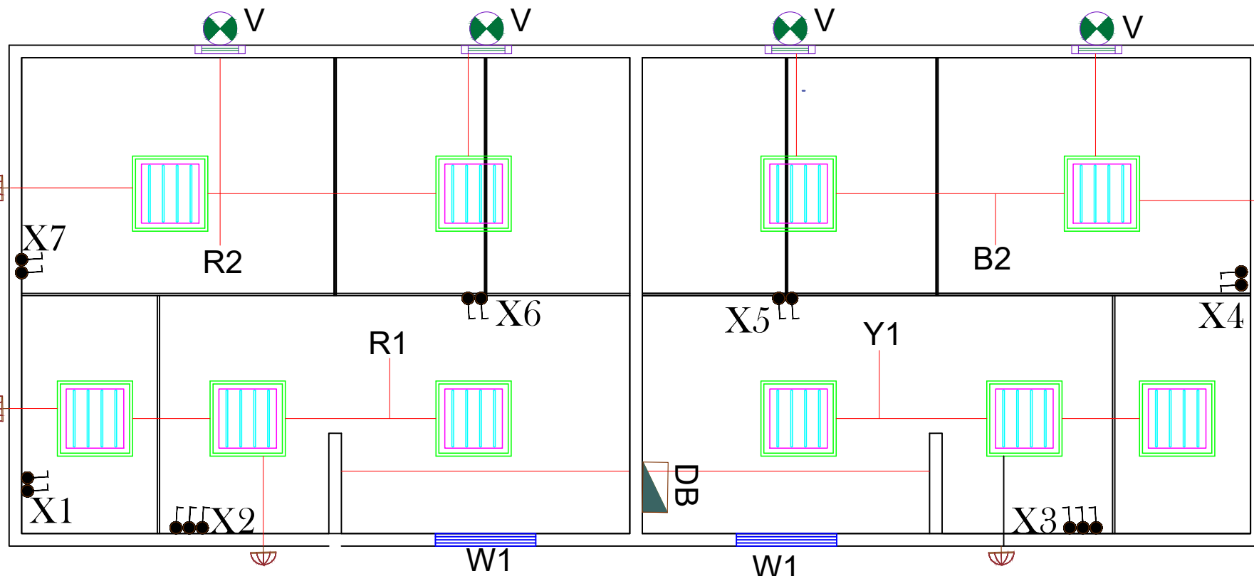
LIGHTING LAYOUT
